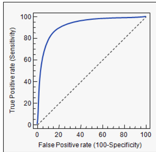
Figure : Area Under the Curve (AUC)
