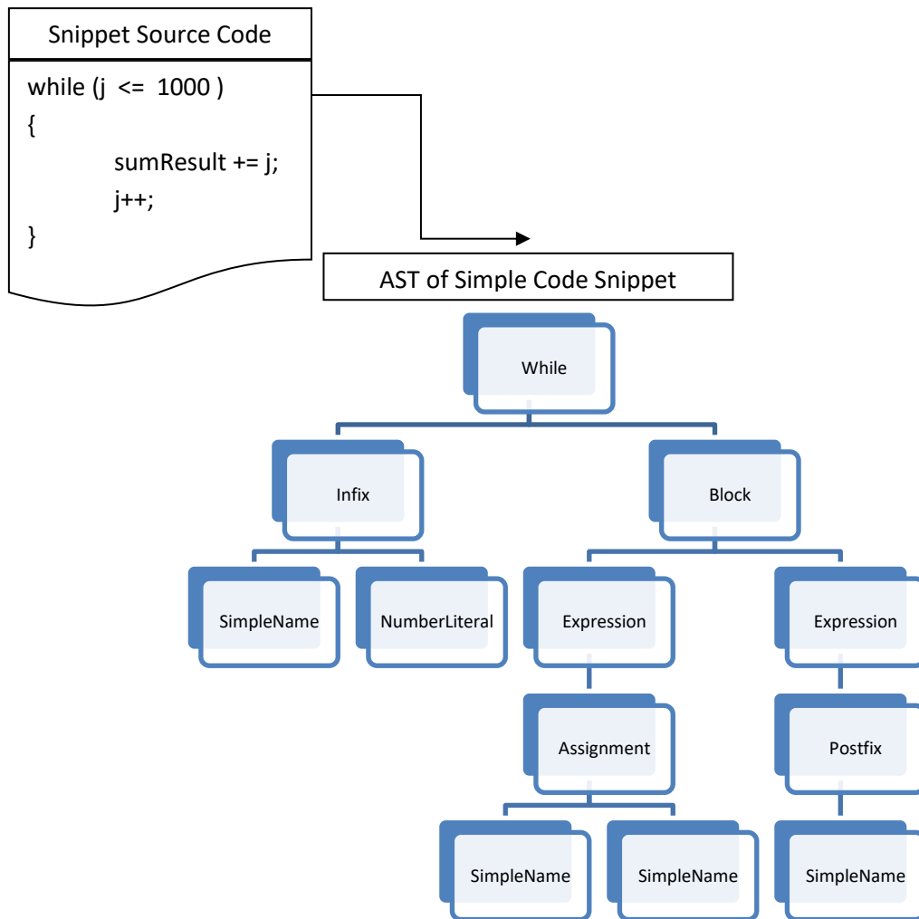
Figure: Source Code Conversion to AST
