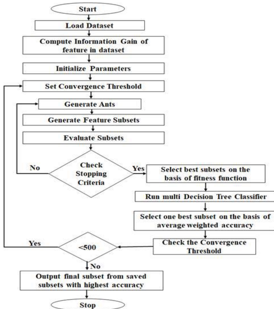
Fig. 1. Proposed Ant Colony – Information Gain Based Feature Selection Method
