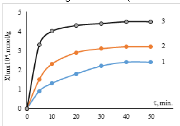
Figure 1. Kinetic curves of the iodine sorption by the fibrous sorbents SMA-3 (1), SMA-1 (2) and SMA-2 (3) at the temperature 40°C. [J_2]=25 mg-equiv/l.
