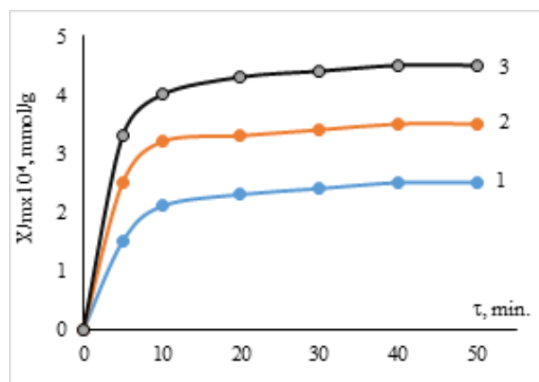
Figure 2. Iodine sorption by SMA-2 sorbent at temperatures 20°C (1), 30°C (2) and 40°C (3). [J_2]=25 mg-equiv/l.
