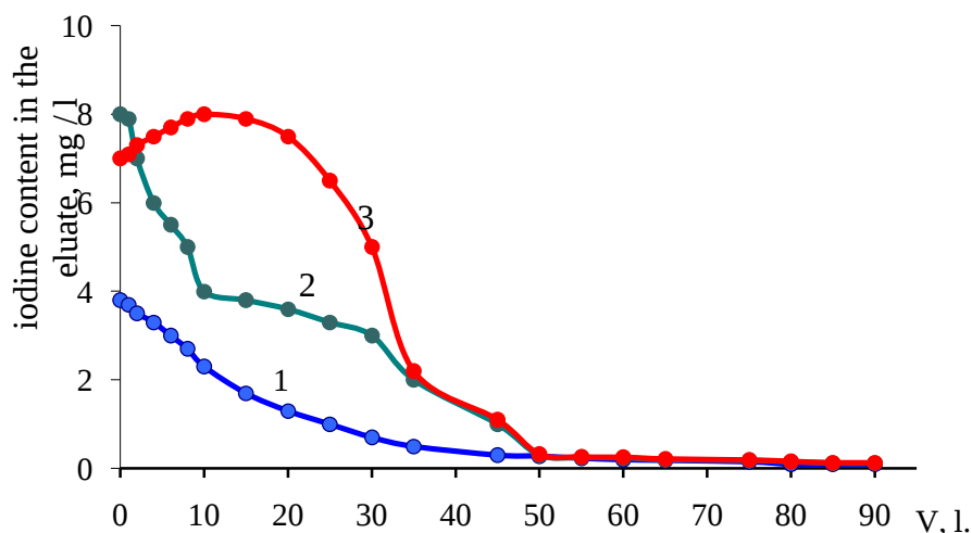
Figure 3. Iodine concentration in distilled water vs volume of the water passed through the layer of sorbents SMA-1 (1), SMA-2 (2) and SMA-3 (3). Iodine content in the sorbents is 3 mg-equiv/g, diameter of the layer 2 cm, fiber mass 5 g, layer height 15 cm, T=25^\circ\text{C} .
